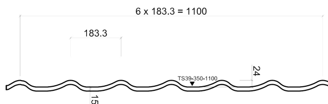
Front section view
